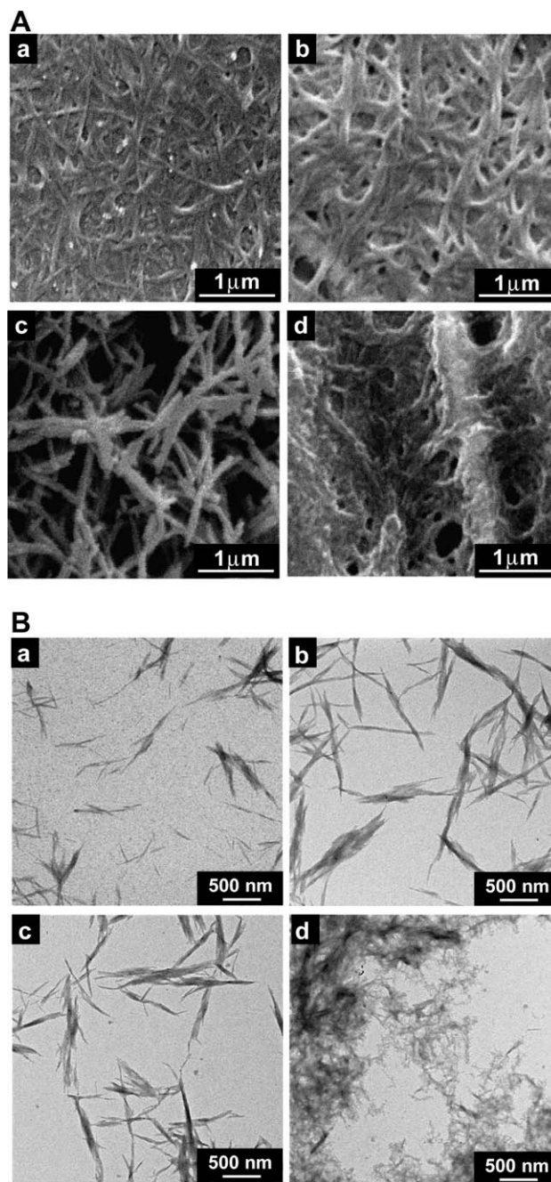
Figure 6. (A) SEM micrographs and (B) TEM micrographs of (a) 2 and 3 under various alkaline concentrations in (b) 40%, (c) 50%, and (d) 60% for 6 h treating time.
