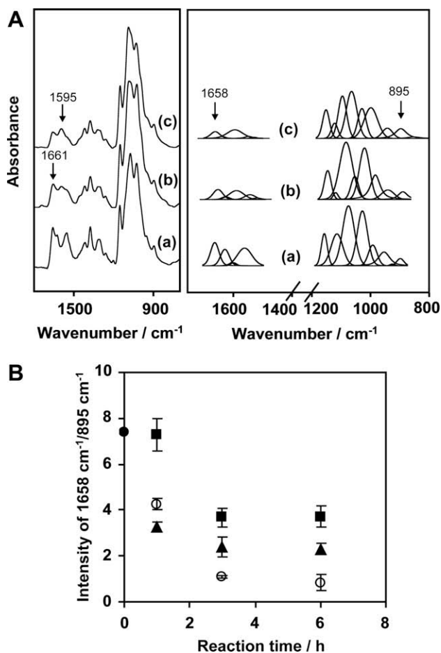
Figure 3. (A) FTIR spectra and curve fitting of 3 in 60% alkaline solution for (a) 1 h, (b) 3 h, and (c) 6 h; and (B) quantitative analysis based on (A) for (●) 2 and 3 under various alkaline concentrations in (■) 40%, (▲) 50%, and (○) 60% for 1, 3, and 6 h treating time.
