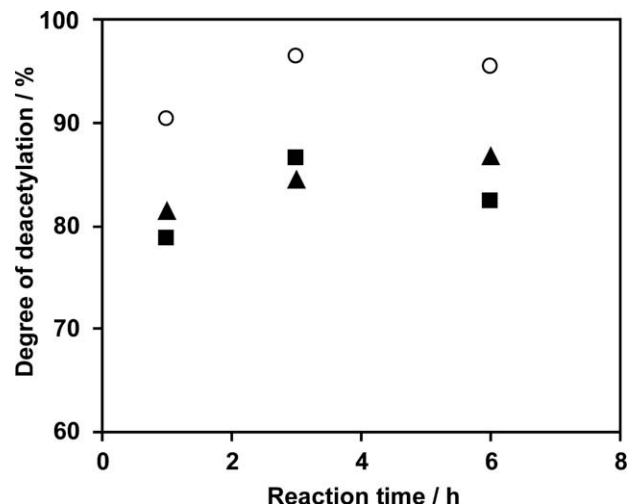
Figure 4. %DD of 3 under various alkaline concentrations in (■) 40%, (▲) 50%, and (○) 60% for 1, 3, and 6 h treating times.
