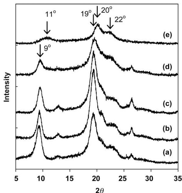
Figure 5. WAXD patterns of (a) 1 , (b) 2 and 3 under various alkaline concentrations in (c) 40%, (d) 50%, and (e) 60% for 6 h treating time.
