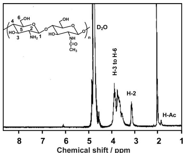
Figure 2. ^1\text{H} NMR spectrum of 3 in 60% alkaline solution for 6 h.
